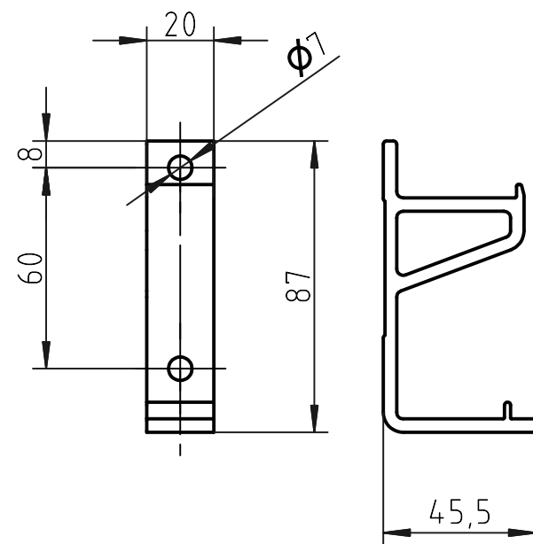
Option B: Cassette bracket for 60mm offset, and adjustable distance brackets
