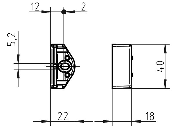
Snap-fit distance bracket (1 : 2)
