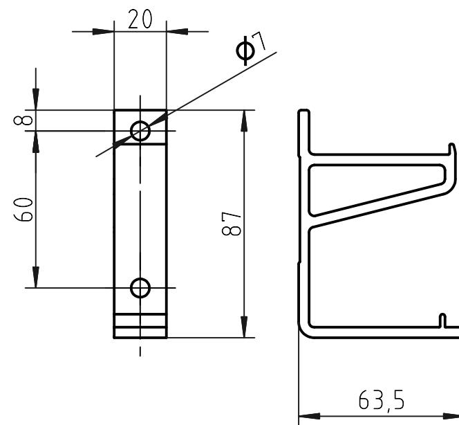
Option C: (1 : 2) Cassette bracket for 80mm offset, and adjustable distance brackets
