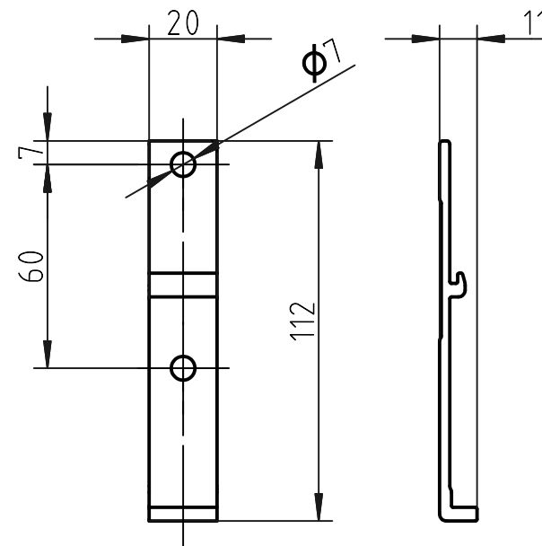
Option A: (1 : 2) Cassette bracket for 27mm offset used with snap-fit distance brackets
