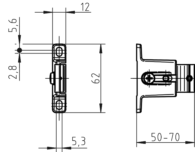
Adjustable distance bracket (1 : 2) (Extension kit available.)
